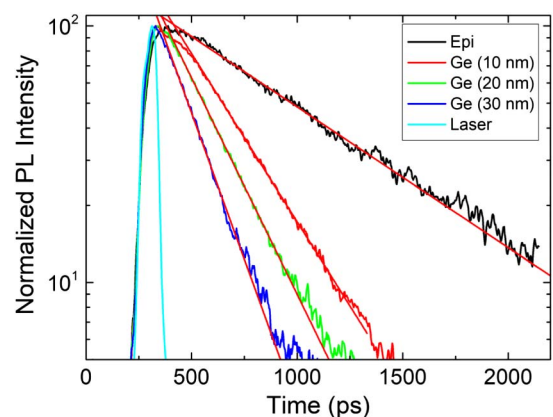
Fig. 3. Measured PL transients from the HMM samples with different Ge thickness (10, 20, and 30 nm). Epi indicates PL decay from an original QD sample, and Laser is for instrument response function.
