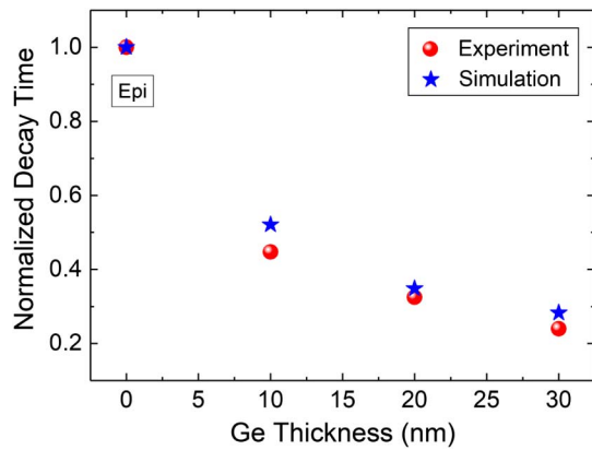
Fig. 4. Comparison of the measured lifetimes of QD exciton (normalized to the value of bare QDs, 790 ps) and the calculated lifetimes for different Ge thickness samples.
