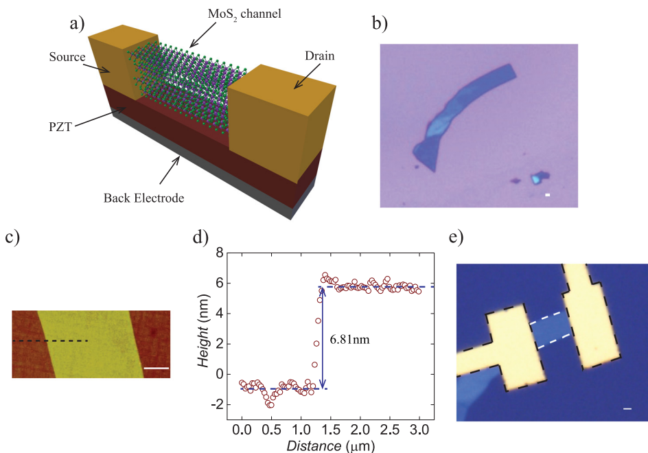
FIG. 2. (a) Schematic of the multilayer \text{MoS}_2 /PZT/SRO back-gate transistor. (b) Optical image of \text{MoS}_2 flake exfoliated onto the 285\ \text{nm}\ \text{SiO}_2/\text{Si} substrate prior to transfer. (c) AFM image of the \text{MoS}_2 flake. (d) AFM result of \text{MoS}_2 flake thickness. (e) Optical image of the back-gate transistor. All scale bars are 1\ \mu\text{m} .
