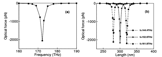
FIG. 4. (a) Spectra of the optical force as a function of the incident frequency, with the geometrical parameters of the system: h=10 nm, l=260 nm, d=50 nm, and the incident intensity of 1.0 \text{ mW}/\mu\text{m}^2 . (b) Spectra of the optical force as a function of length of nanorod for three incident wave with frequency f=144.4 THz, 152.6 THz, and 161.8 THz, with the geometrical parameters of the system: h=10 nm, d=50 nm, and the incident intensity of 1.0 \text{ mW}/\mu\text{m}^2 .
