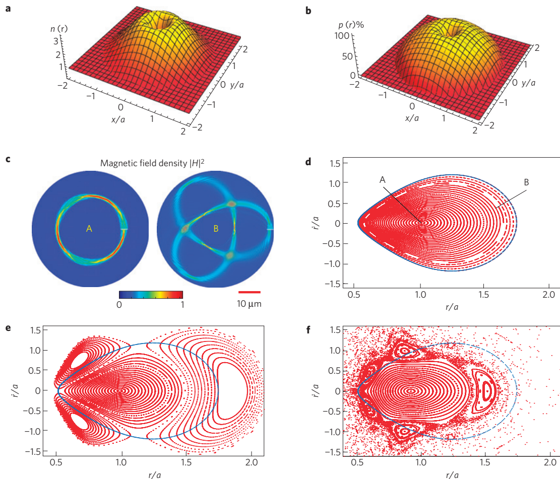
Figure 3 | CIPTs based on air-GaInAsP composite media. a, b Refractive index profile ( a ) and volume fraction ( b ) of the GaInAsP. c , FDFD simulations of bound and stable light propagation in the form of A, a circular orbit with period 2\pi and B, a 'Rosetta' type of orbit with period 4\pi . In the calculations, a linear source with width w = 6\lambda and wavelength \lambda = 1.55 \mu\text{m} is used. d-f , Poincaré maps ( P_T ) corresponding to all possible photon trajectories for linear ( d ) and nonlinear ( e, f ) refractive indices. In the linear case, the photon motion follows stable periodic and quasi-periodic trajectories for all initial conditions. With the introduction of nonlinearity, the stability of the system is disturbed with some trajectories passing through the cavity boundaries and leaving the system. f , For above-critical values of the nonlinear index \Delta n_{\text{NL}}/n_{\text{max}} = 0.2 , chaotic behaviour is observed similarly to the three-body problem in celestial mechanics. In generating the Poincaré maps, the scale-invariant parameters r/a and \dot{r}/a are sampled at times t_m = 2\pi m/\omega_{\text{NL}} that are an integer number m of the nonlinear period (or T-period map), and the derivative is taken with respect to the azimuth angle \varphi .
